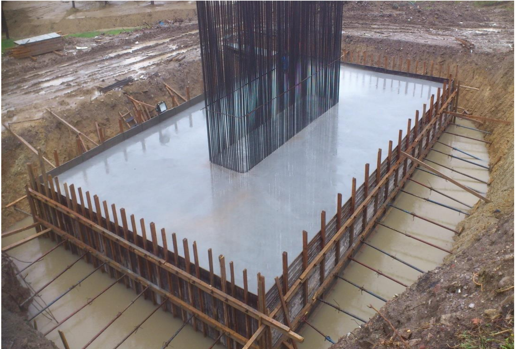
VIADUCT FOUNDATION
